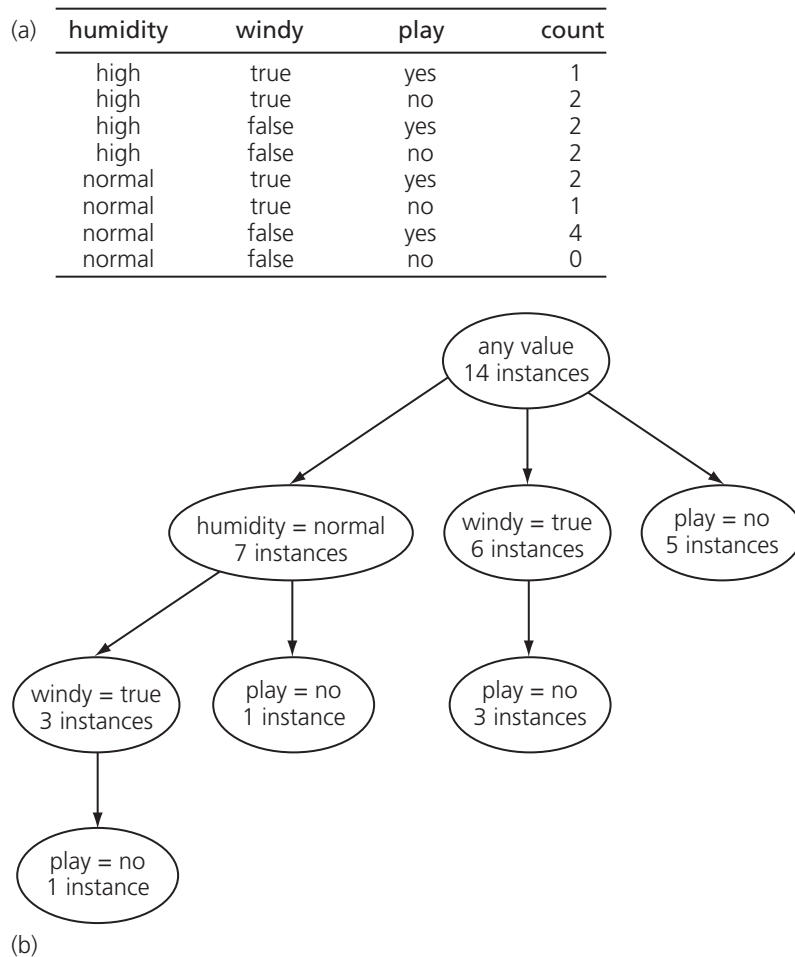
Figure 6.22 The weather data: (a) reduced version and (b) corresponding AD tree.
